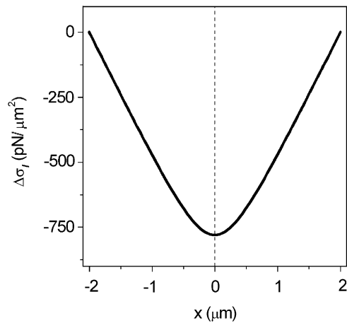
Fig. 2. The change of longitudinal stress in the CM due to DNA strings according to Eq. (5) with the following parameters: R = 0.5 \mu\text{m} , r = 0.25 \mu\text{m} , a = 1 \mu\text{m} , b = 2 \mu\text{m} , t = 20 \text{ nm} , N = 10 , f = 1 \text{ pN} .
