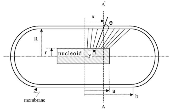
Fig. 1. The modified TOW model of a bacillary bacterium. The membrane is composed of two layers, cytoplasmic (inner) and peptidoglycan (outer). The straight lines connecting the nucleoid to the CM represent the DNA/mRNA/m-proteins strings. Strings in the first quadrant only are displayed; those not shown, present in the other quadrants, preserve the symmetry of the cell.
