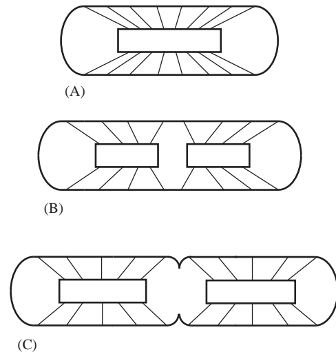
Fig. 3. A schematic transition from a minimum tensile stress to zero at the midpoint of a cell during nucleoid separation. (A) Before separation—the midpoint is under minimum stress. (B) In the initial stage of nucleoid separation—stress at midpoint is around zero. (C) After separation—midpoint stress vanishes.
